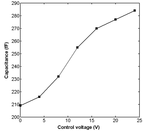
Figure 6. Measured tuning characteristic of the 1 st generation tunable capacitor designs in Agilent 0.5 \mu\text{m} CMOS process.
