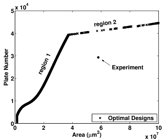
Figure 3. Pareto front for 41 section serpentine design
