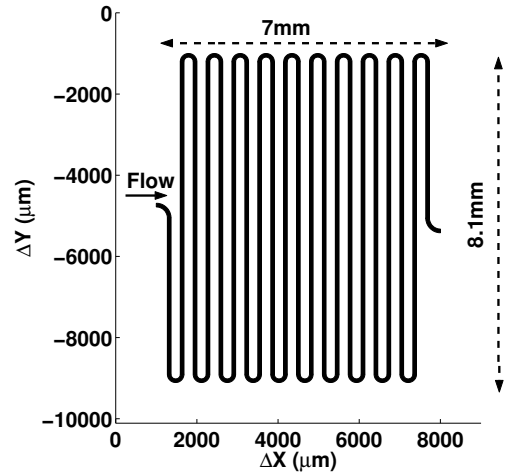
Figure 2. Schematic of Serpentine by Jacobson et al. (1994)
