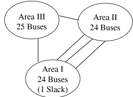
Fig. 5. IEEE RTS-1996 system sketch
