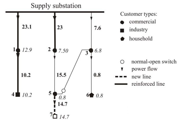
Fig. 2. Optimal Solution for 10 Years Planning Period - (a)
