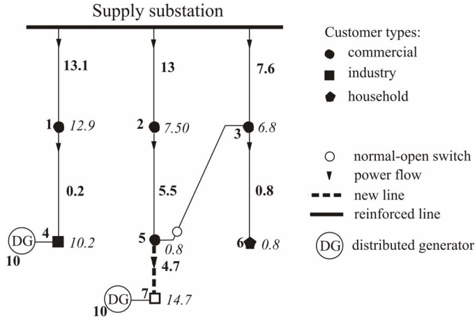
Fig. 4. Optimal Solution for 10 Years Planning Period - (c)
