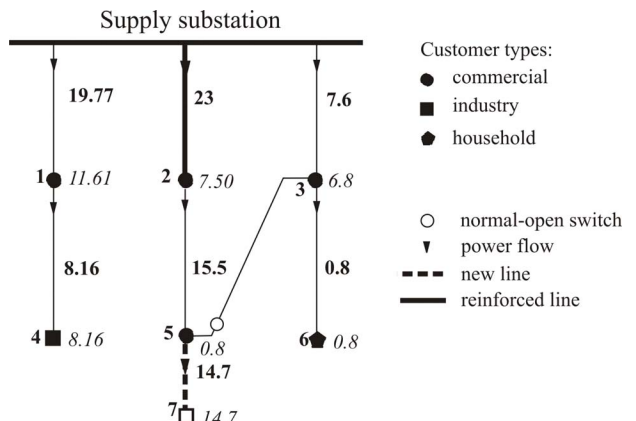
Fig. 3. Optimal Solution for 10 Years Planning Period - (b)
